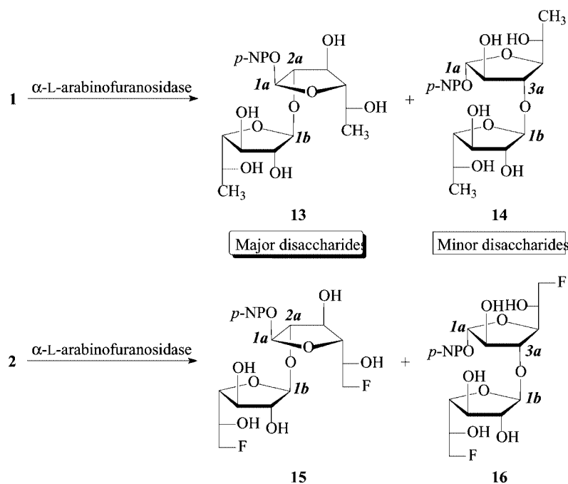
Figure 3. Structures of disaccharides 13 , 14 and 15 , 16 obtained from the AbfD3-catalysed condensation of 1 and 2 , respectively.
