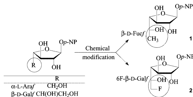
Figure 1. Chemical structures of targeted 6-modified galactofuranosides 1 and 2 .
