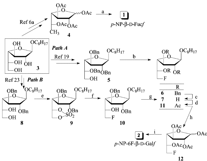
Scheme 1. (a) i. p -NPOH, \text{BF}_3 \cdot \text{OEt}_2 , \text{Et}_3\text{N} , \text{CH}_2\text{Cl}_2 ; ii. \text{MeONa} , \text{MeOH} (66%); (b) DAST, \text{Et}_3\text{N} , \text{CH}_2\text{Cl}_2 (47%); (c) \text{NaBrO}_3 , \text{Na}_2\text{HSO}_3 , \text{H}_2\text{O} , \text{AcOEt} (80%); (d) \text{Ac}_2\text{O} , \text{Pyr} (97%); (e) i. \text{SOCl}_2 , \text{Pyr} , \text{CH}_2\text{Cl}_2 ; ii. \text{RuCl}_3 , \text{NaIO}_4 , \text{CH}_3\text{CN} , \text{H}_2\text{O} , \text{CH}_2\text{Cl}_2 (89%); (f) i. TBAF, \text{THF} , \text{Me}_2\text{CO} ; ii. \text{H}_2\text{SO}_4 , \text{H}_2\text{O} (86%); (g) \text{H}_2 , \text{Pd}(\text{OAc})_2 , \text{AcOH} , \text{AcOEt} (92%) (h) \text{Ac}_2\text{O} , \text{H}_2\text{SO}_4 , \text{CH}_2\text{Cl}_2 (98%); (i) i. p -NPOH, \text{BF}_3 \cdot \text{OEt}_2 , \text{Et}_3\text{N} , \text{CH}_2\text{Cl}_2 ; ii. \text{MeONa} , \text{MeOH} (61%).
