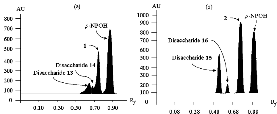
Figure 2. HPTLC chromatograms at 300 nm for the AbfD3-catalysed transformations of 1 (a) and 2 (b).
